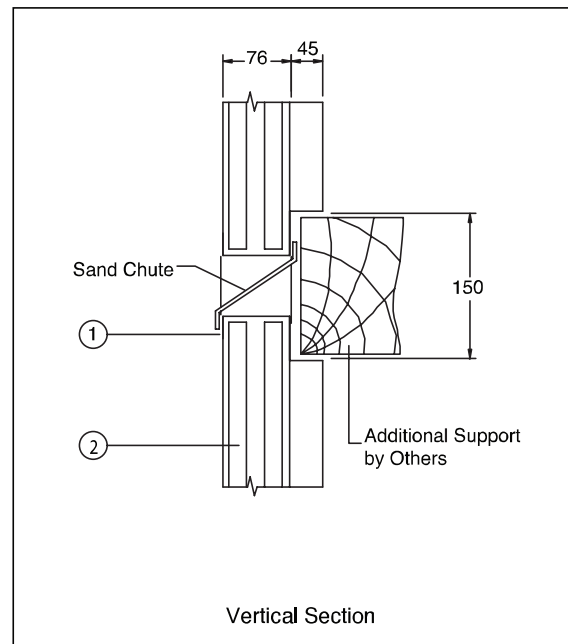
Multiple Section with Sand Chute
