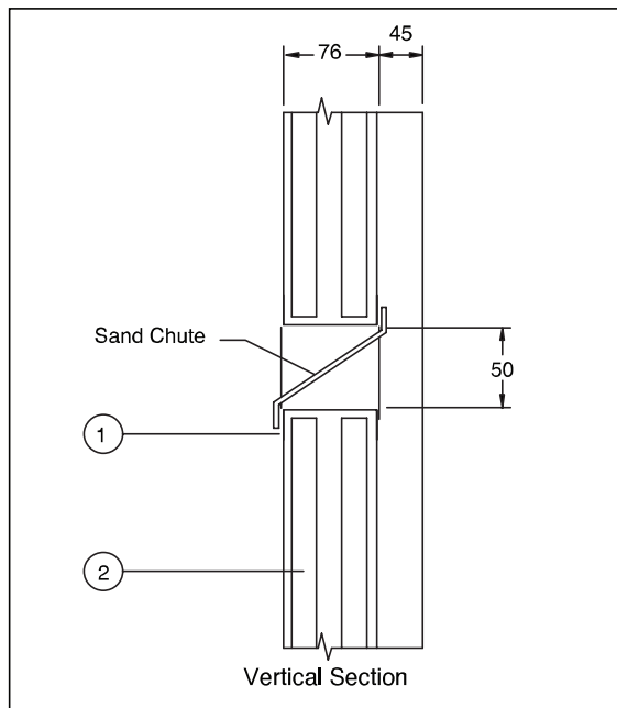
Single Section with Sand Chute
