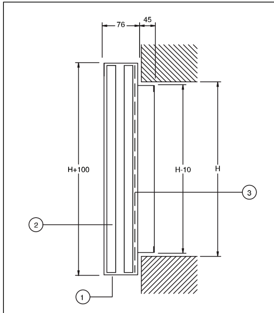
Vertical Section
