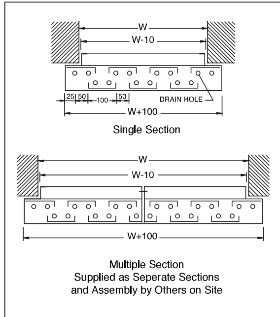
Horizontal Section
